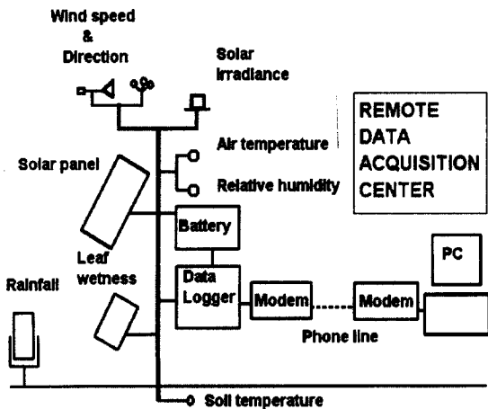
Fig. 2. Schematic diagram of the hardware components automated weather stations.
