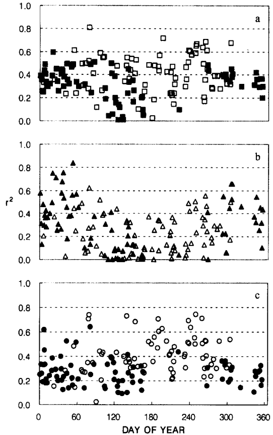
Fig. 2. Coefficients of determination for the simple linear regression of the observed daily average (top), maximum (middle), and minimum (bottom) temperature to the station elevation. Solid and empty symbols indicate clear (cloud amount < 2) and overcast (cloud amount > 8) sky conditions, respectively.
