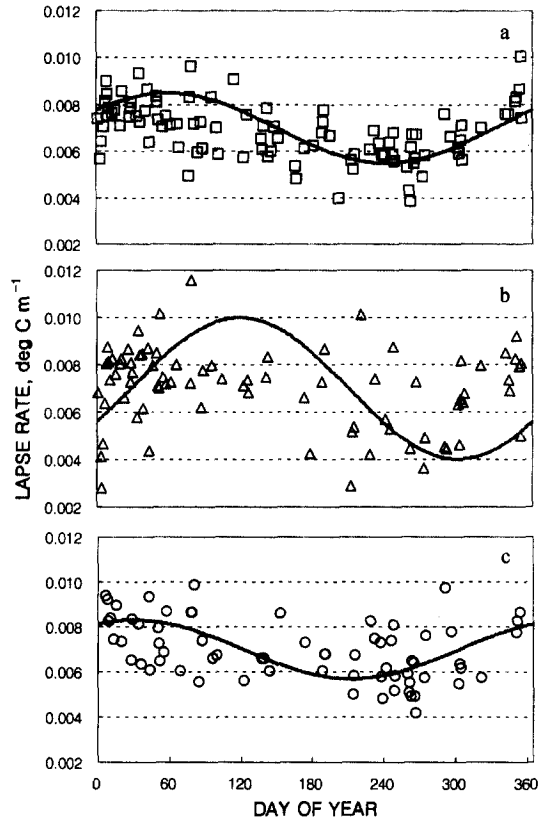
Fig. 4. Scatter plot of the partial regression coefficients of station elevation in the daily average (top), maximum (middle), and minimum (bottom) temperature models. The sinusoidal lines were manually fitted for the corresponding scatter plots.
