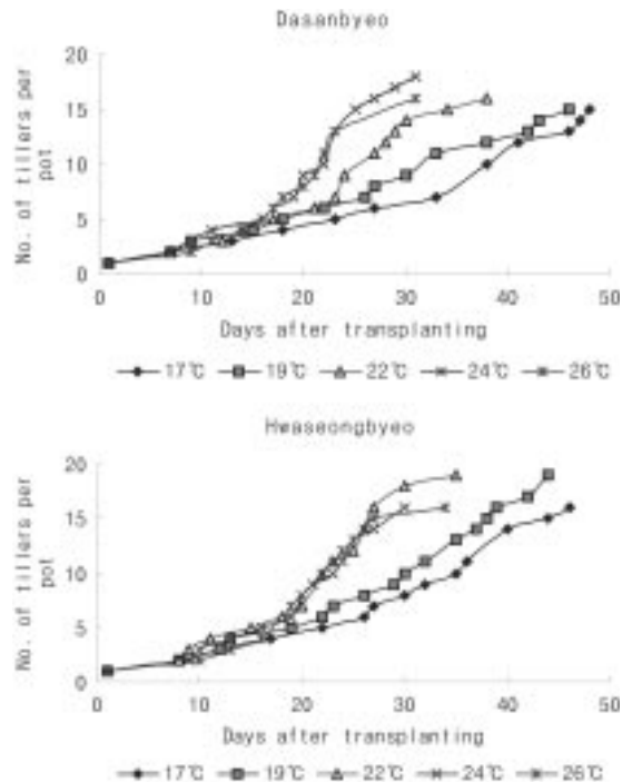
Fig. 2. Time course changes of tillers affected by different temperature conditions in rice plant.
