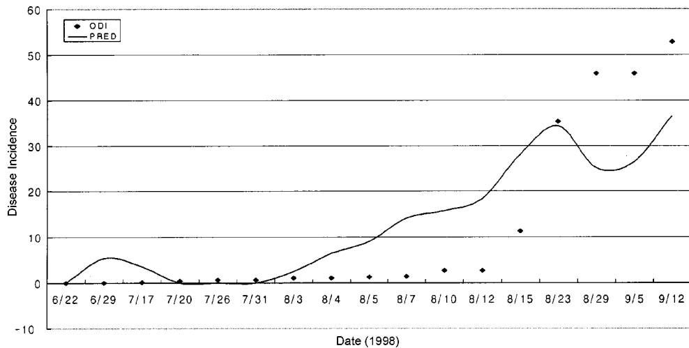
Fig. 2. Observed and predicted disease incidence(DI) values of disease progress curve on Phytophthora blight in red pepper at the Field plot.
