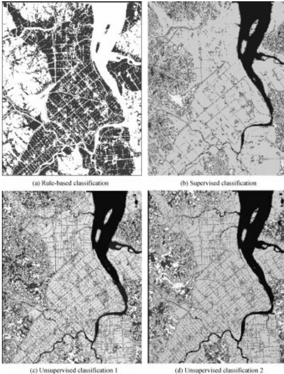
Fig. 5. Paddy field area extracted by four different methods.
