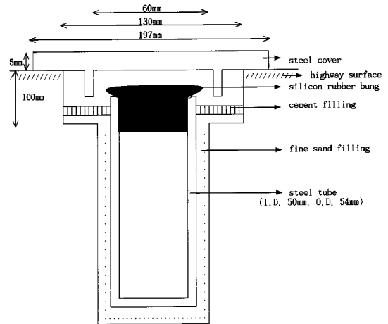
Fig. 1. Schematic diagram of access tube for neutron moisture meter.
