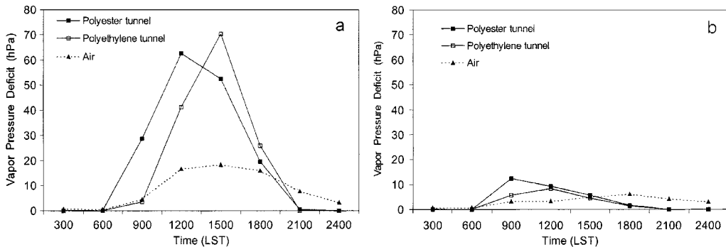
Fig. 3. Diurnal variation of vapor pressure deficit for polyester tunnel, polyethylene tunnel, and ambient air on sunny(a) and cloudy with rain(b) day in 1999 at Suwon.
