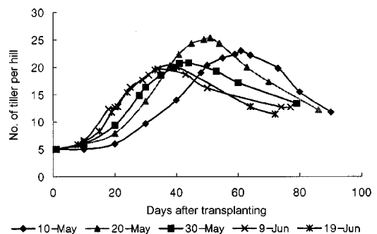
Fig. 1. Time course change of the tiller number affected by different transplanting dates of Dasanbyeo rice.
