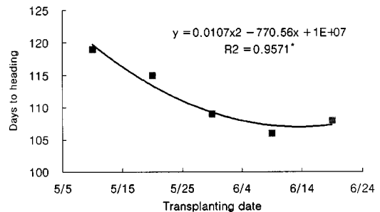
Fig. 2. Change in growth duration from seeding to heading affected by different transplanting date of Dasanbyeo rice.
