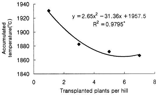
Fig. 3. Relationship between the accumulated temperature from transplanting to heading and the transplanted plants per hill of Dasanbyeo rice.
