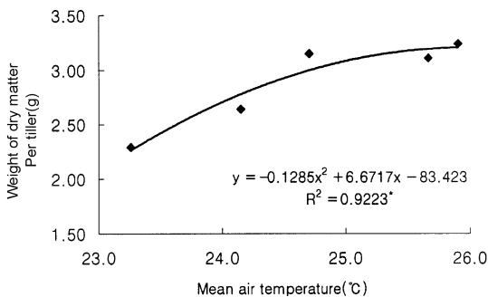
Fig. 6. Relationship between weight of dry matter per tiller at heading stage and mean air temperature from transplanting to heading date of Dasanbyeo rice.
